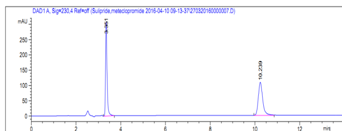
Figure 4: HPLC chromatogram of rabbit plasma containing Sulpiride and Metoclopramide.
