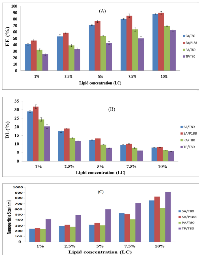
Figure 1: Effect of lipid type and lipid concentration (LC) on EE (A), DL (B) and nanoparticle size (C) of SLNs prepared with different lipid, lipid concentration (LC) and surfactant (S) using 2% soy lecithin as co-surfactant.
