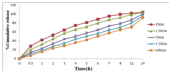
Figure 3: Effect of lipid concentration on the release of Sulpiride from SLNs prepared with 2% Soya lecithin as co-surfactant.
