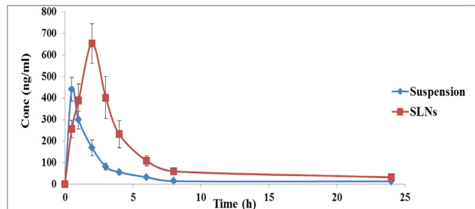
Figure 5: Mean plasma concentration of Sulpiride after oral administration of Sulpiride suspension (10mg/ml) and Sulpiride SLNs.
