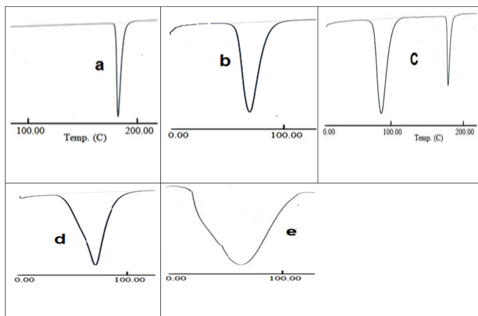
Figure 2: DSC spectra of: a) Sulpiride, b) Stearic acid, c) Stearic acid + Sulpiride PM, d) Blank SLNs, e) Sulpiride SLNs.
