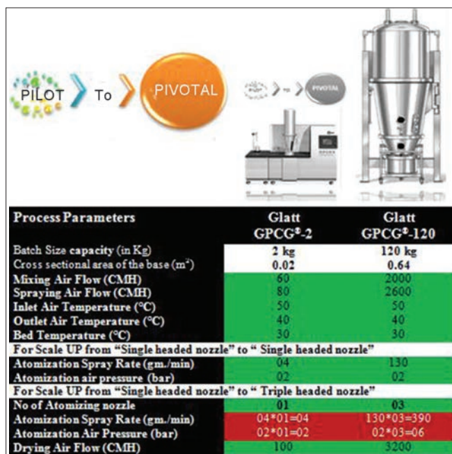
Figure 8: Controlled FBP Parameters from small lab scale to large production scale
