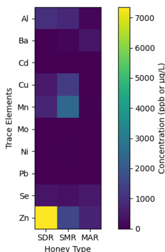
Figure 2: Heatmap showing the distribution of trace element concentrations in Sidr Honey ( Ziziphus spina-christi L.; SDR), Samar honey ( Acacia tortilis ; SMR), and Maraee honey (multifloral origin; MAR) determined by ICP-MS. Color intensity corresponds to element concentrations (ppb or µg/L). SDR is characterized by high Zn levels, SMR by elevated Cu and Mn, and Maraee by relatively higher Ba and Se concentrations, indicating distinct elemental profiles associated with botanical and geographical origin.
