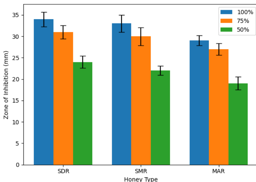
Figure 1: Antibacterial activity of Sidr Honey ( Ziziphus spina-christi L.; SDR), Samar honey ( Acacia tortilis ; SMR), and Maraee honey (multifloral origin; MAR) against Methicillin-resistant Staphylococcus aureus (MRSA) at different concentrations. Bars represent the mean Zone of Inhibition (ZOI) obtained from replicate experiments, while error bars indicate the Standard Deviation (SD). The inhibition zones decreased with decreasing honey concentration, with SDR and SMR showing greater antibacterial activity than MAR.
