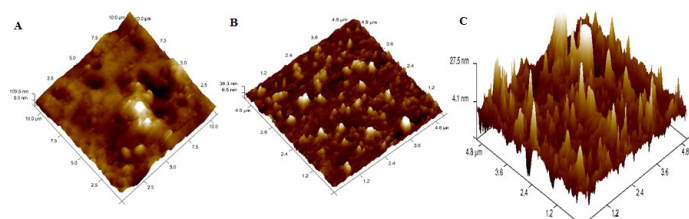
Figure 3: Atomic Force Microscopy (A-CLR, B-CCLR and C-SLR).
