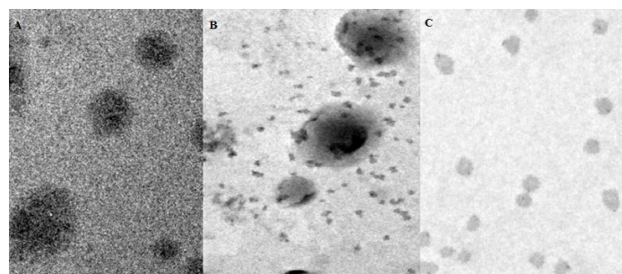
Figure 2: Transmission Electron Microscopy (A-CLR, B-CCLR and C-SLR).
