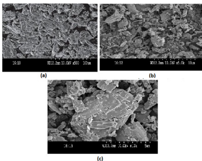
Figure 3: SEM images of PL7 formulation.
