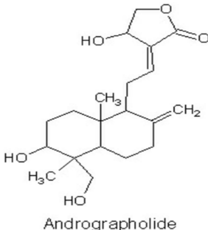
Figure 2: Structure of andrographolide.
