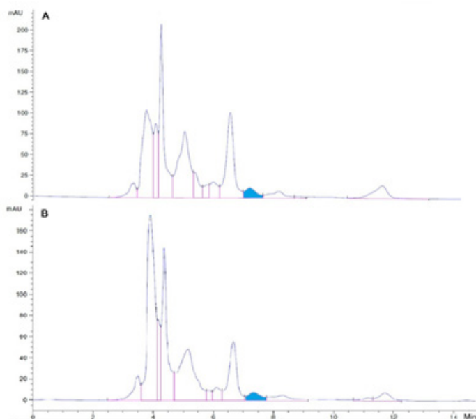
Figure 3: HPLC chromatograph determining andrographolide content (blue shaded peak areas) from, A: A. paniculata extract in 33% acetic acid; B: Oxymel formulated containing A. paniculata extract and honey.
