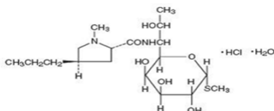
Lincomycin hydrochloride
