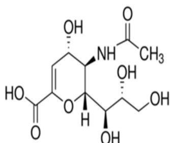
N-Acetyl-1,2,3-dehydro-2-deoxyneuraminic acid
